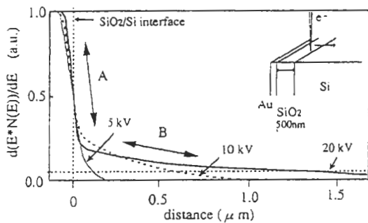
Fig. 2. O KLL intensity distribution on the cross section of Au/SiO 2 /Si specimen. (beam current: 10 nA)
