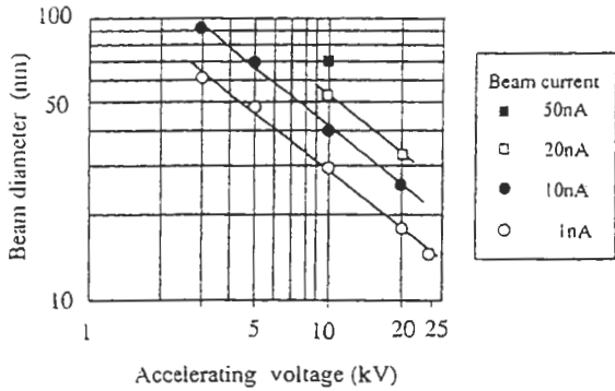
Fig. 1. Dependence of beam diameter on accelerating voltage.
